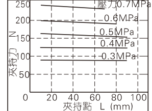
HFSZ40\HFSK40
