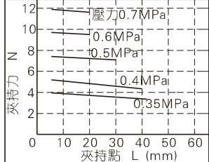
HFTZ16\HFTK16
