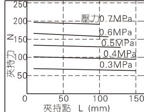
HFTZ40\HFTK40
