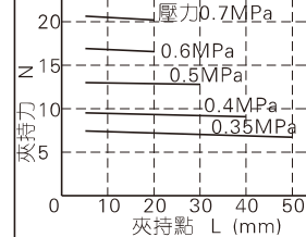
HFSZ16\HFSK16
