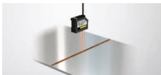
Detect welding seams on steel plates. The Height Difference Count Filter Function enables stable detection.
