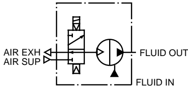
Built-in solenoid valve
