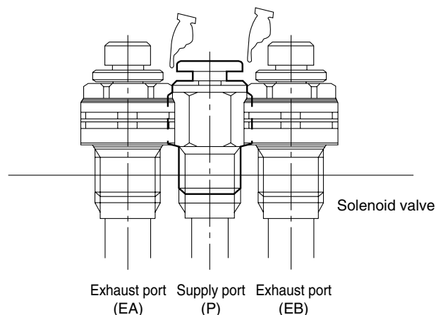
Fig. Example of the interference with fittings
