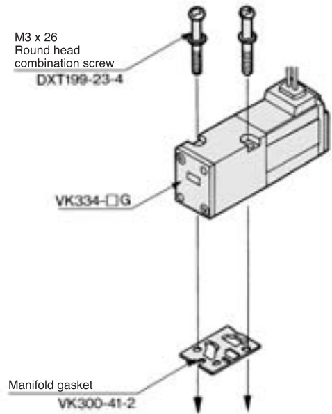
3 port base mounted: VK334
