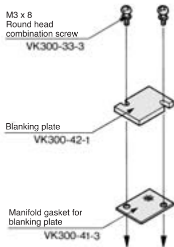
Blanking plate assembly: VK300-42-1A
