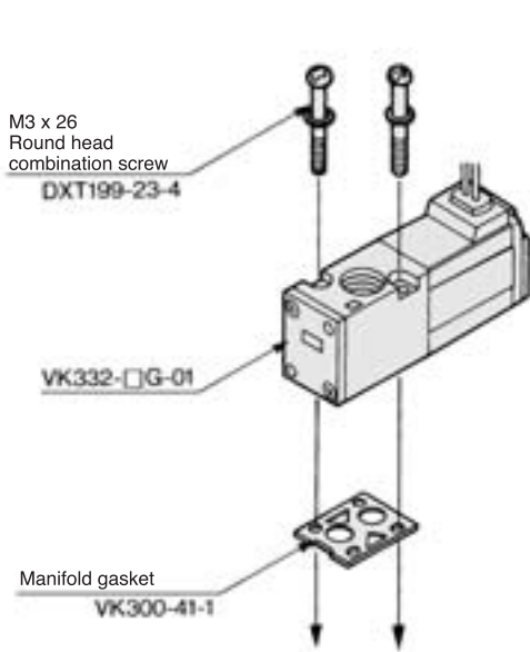
3 port body ported: VK332
