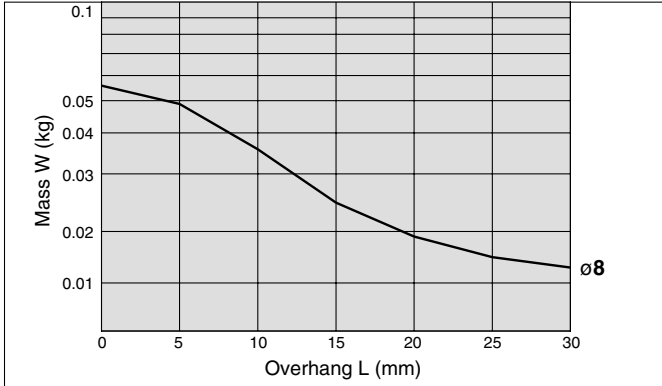
Graph (12) Stroke: Up to 20 stroke
