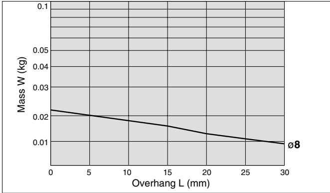
Graph (13) Stroke: Up to 30 stroke
