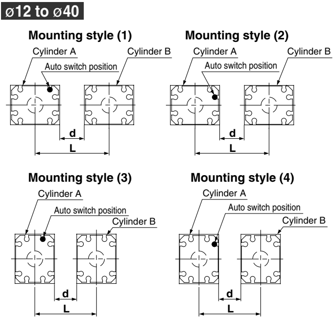
Dimensions by Mounting Style
