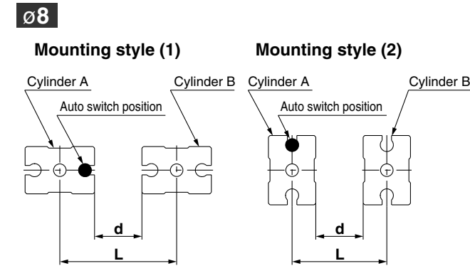
Dimensions by Mounting Style
